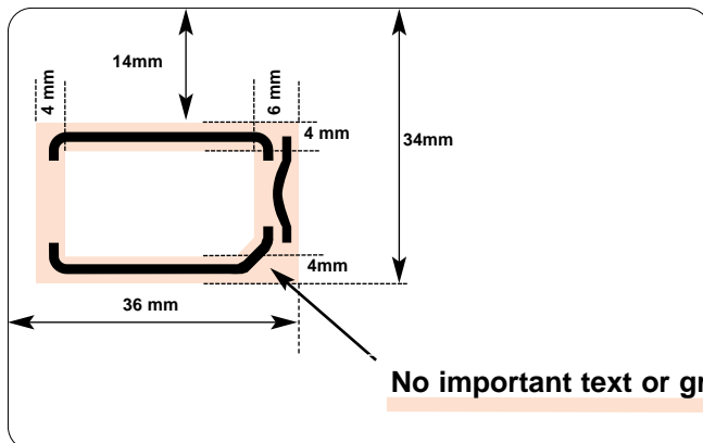
Front /GSM Cards with Plug-In zone
